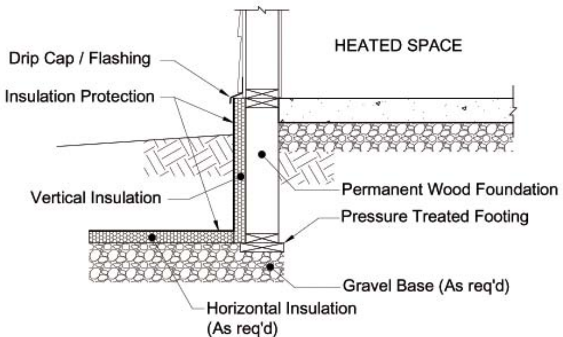
Figure 12. Typical Permanent Wood FPSF
