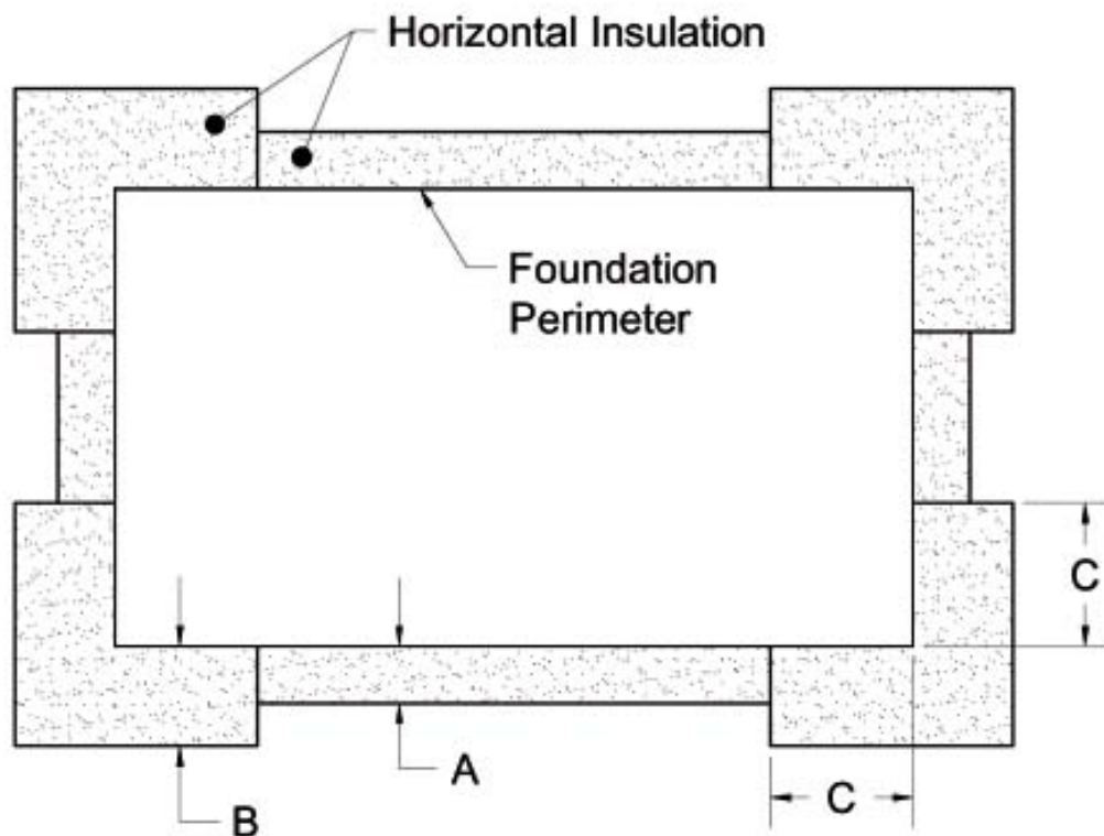
Figure 5. FPSF Simplified Design Parameters – Heated Buildings
