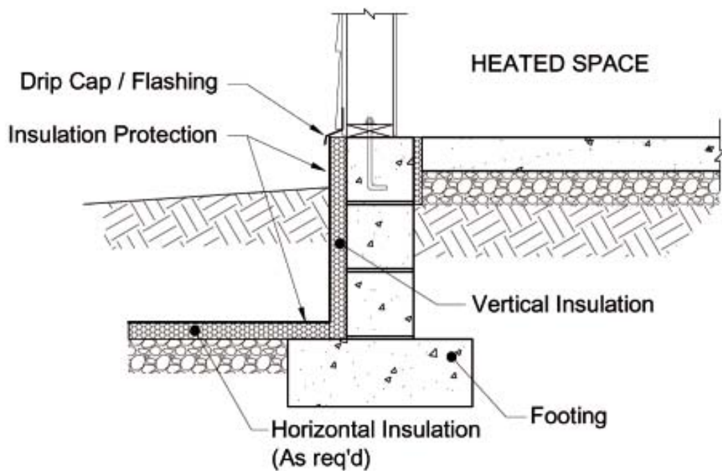
Figure 11. Independent Block Stem Wall
